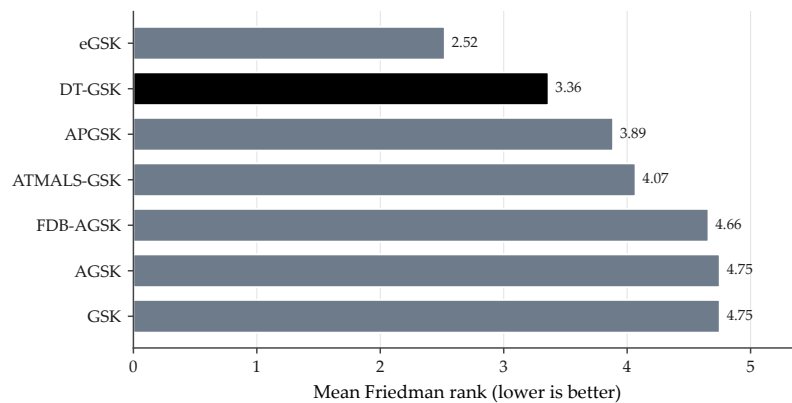
Figure 5. Friedman mean ranks over the 22 CEC2011 real-world problems (25 runs each, raw best-fitness basis), sorted best-first; DT-GSK highlighted. Lower is better. Within this panel DT-GSK’s across-problem Wilcoxon vs. eGSK is a significant loss (Holm p = 4.2 \times 10^{-2} ).
