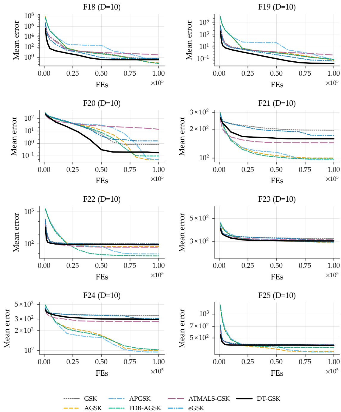
Figure B5. Family-overlap convergence on CEC2017 at D = 10 , functions F18–F25 (sub-grid c of 4): per-checkpoint mean error across 51 runs per algorithm, 7-curve overlay, log-error y-axis (display floor 10^{-14} ), one shared legend. APGSK checkpoint evidence at this dimension derives from per-generation logs (disclosed limitation).
