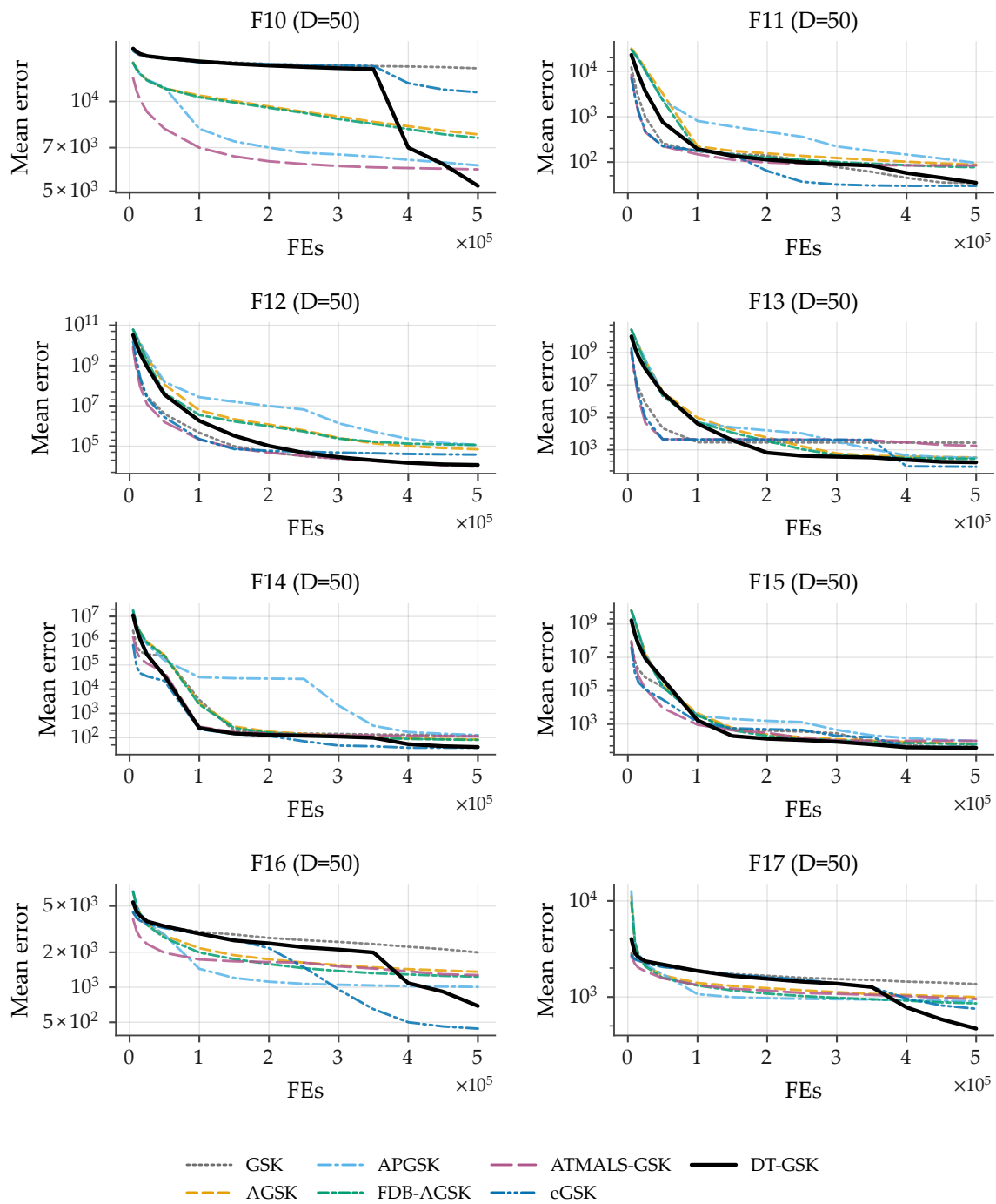
Figure B12. Family-overlay convergence on CEC2017 at D = 50 , functions F10–F17 (sub-grid b of 4): per-checkpoint mean error across 51 runs per algorithm, 7-curve overlay, log-error y-axis (display floor 10^{-14} ), one shared legend. APGSK checkpoint evidence at this dimension derives from per-generation logs (disclosed limitation).
