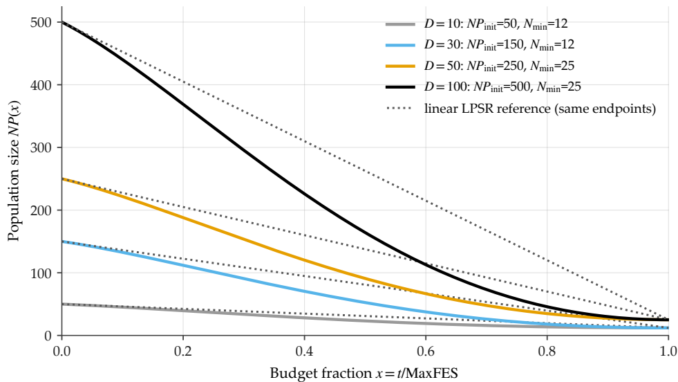
Figure B26. Analytic trajectory of the tier-floored nonlinear population size reduction schedule under the frozen configuration for all four dimension tiers ( NP_{\text{init}} = 5D ; N_{\text{min}} = 12/12/25/25 ): population size vs. consumed budget fraction. Analytic evaluation of the frozen formula — no empirical result values.
