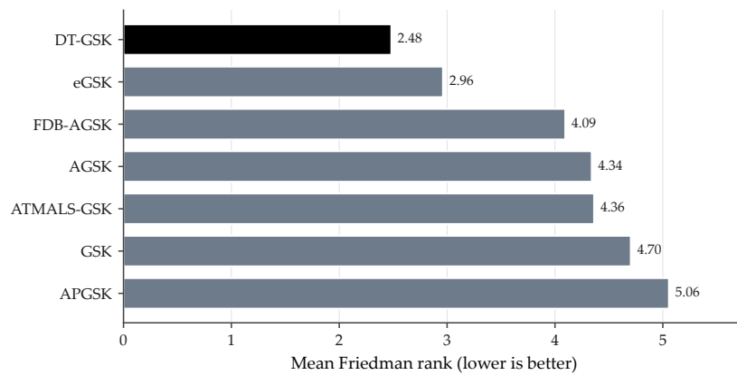
Figure B1. Overall (dimension-aggregated) Friedman mean rank of the seven GSK-family algorithms on CEC2017; lower is better. Same ranks, qualifications, and provenance as the main paper’s family-panel rank table.
