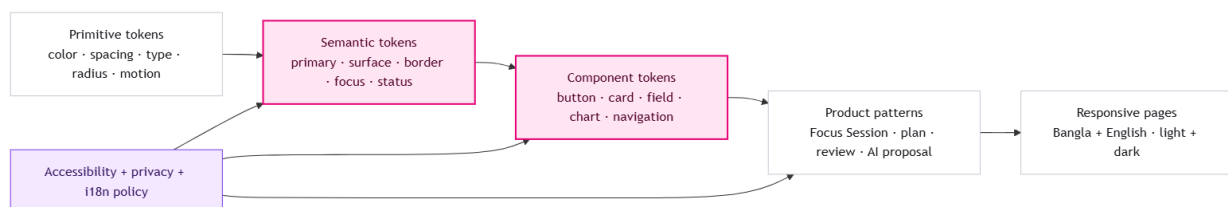
Token architecture
