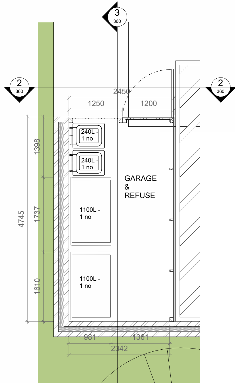
1 Proposed Ground FFL - Refuse 1 : 50
