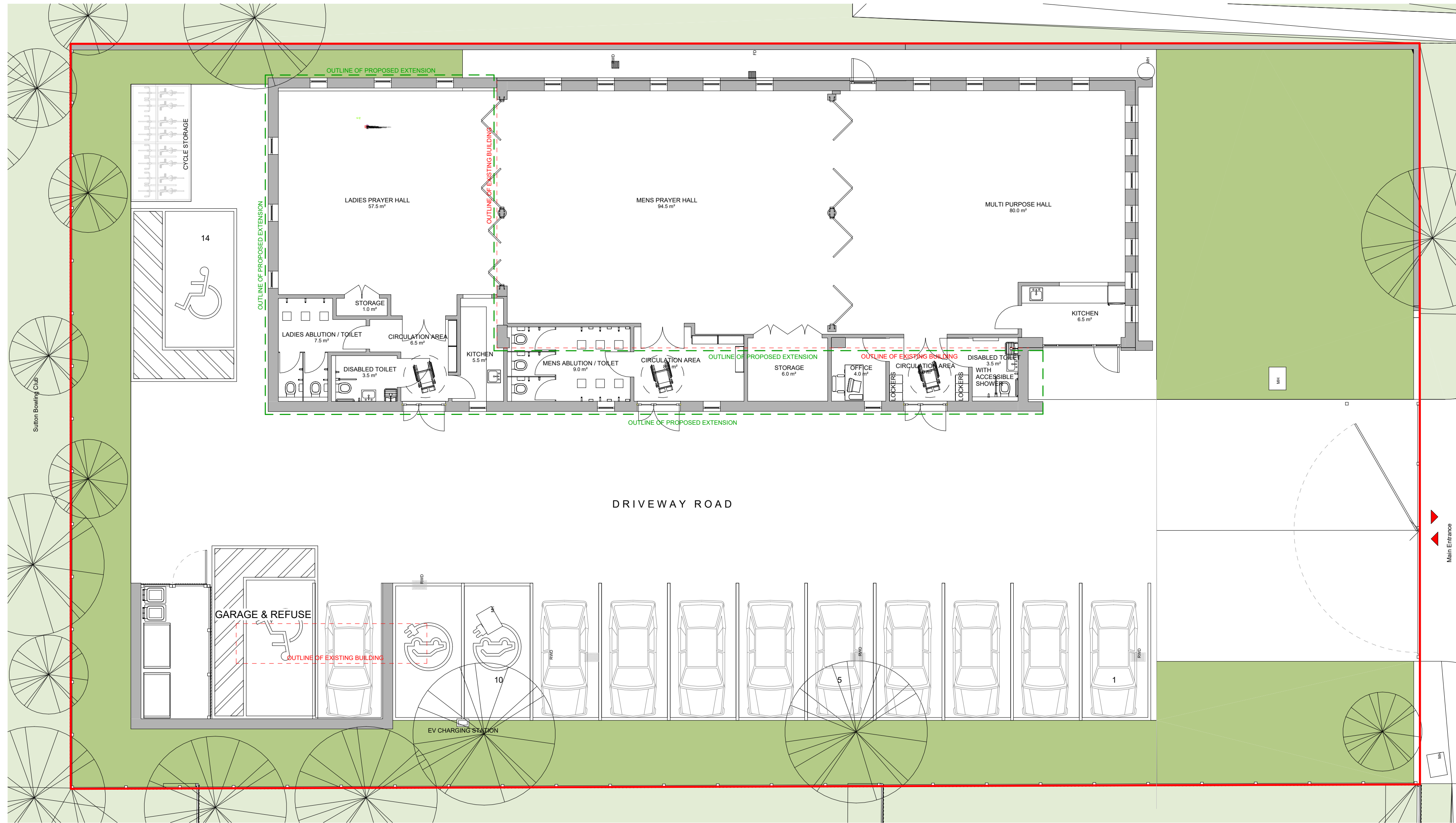
1 Proposed Site Layout Plan 1 : 100
