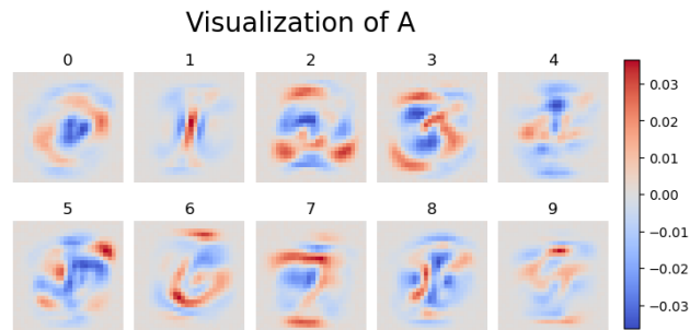
Figur 3: Visualization of the weights matrix at 5 epochs with batches of size 2000.
