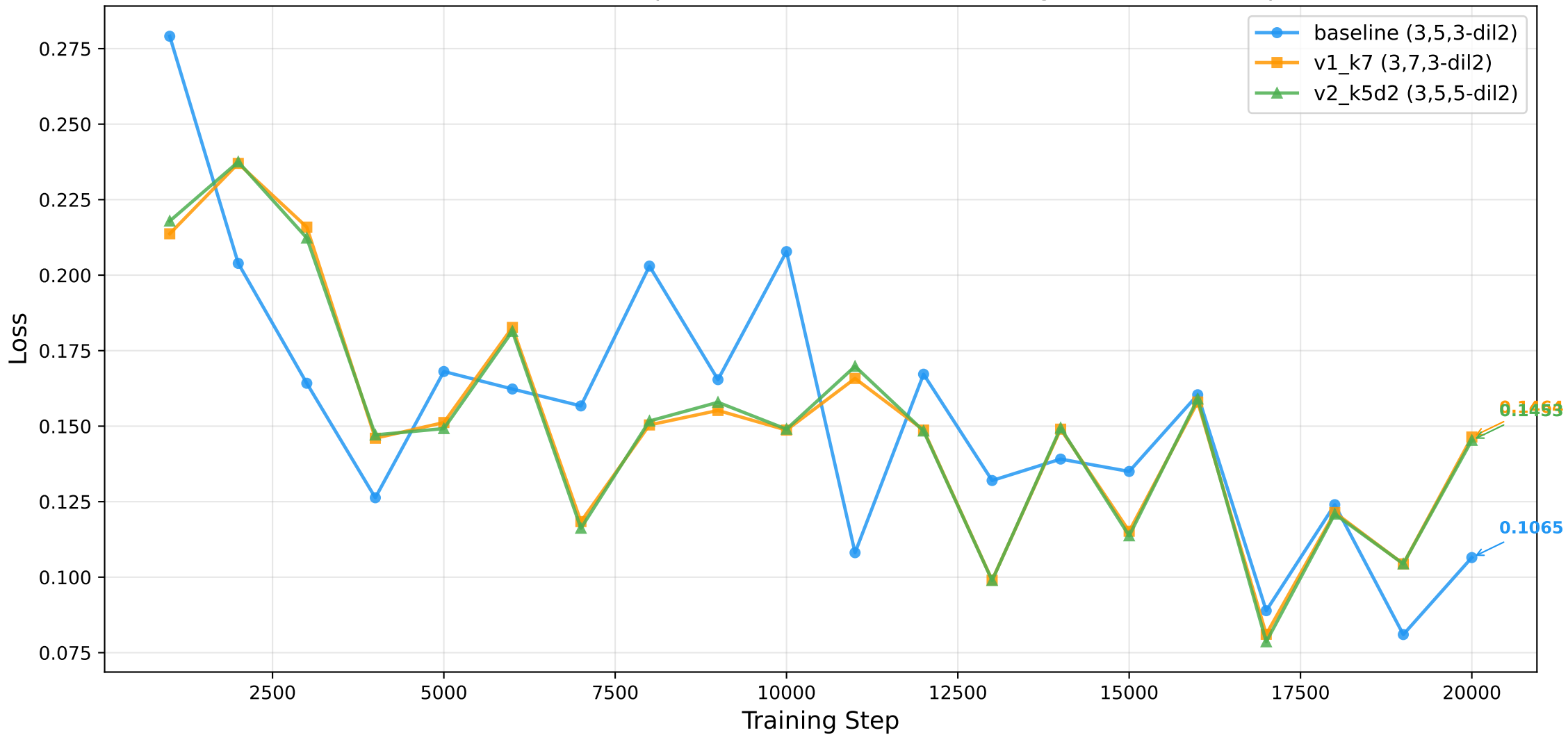
PlanOne Multi-Scale Temporal Conv Variants — Training Loss (20000 steps)
