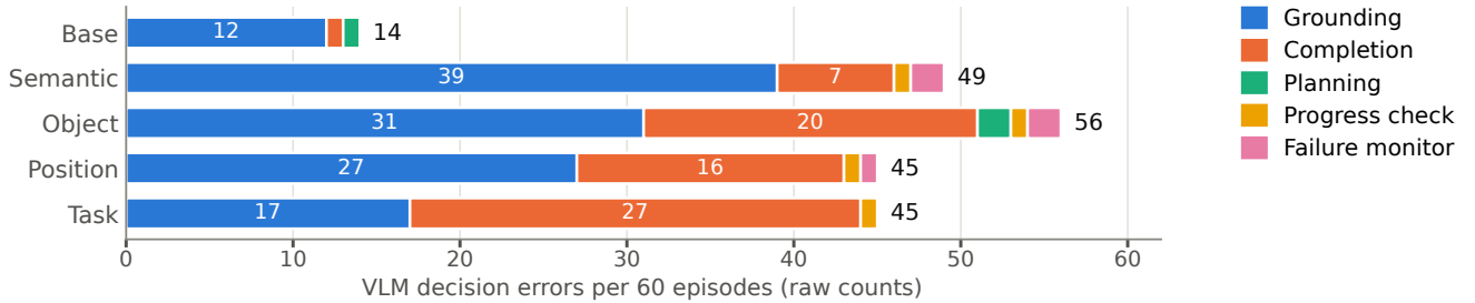
Figure 7. Failure analysis of VLM decision errors across LIBERO-PRO settings.
