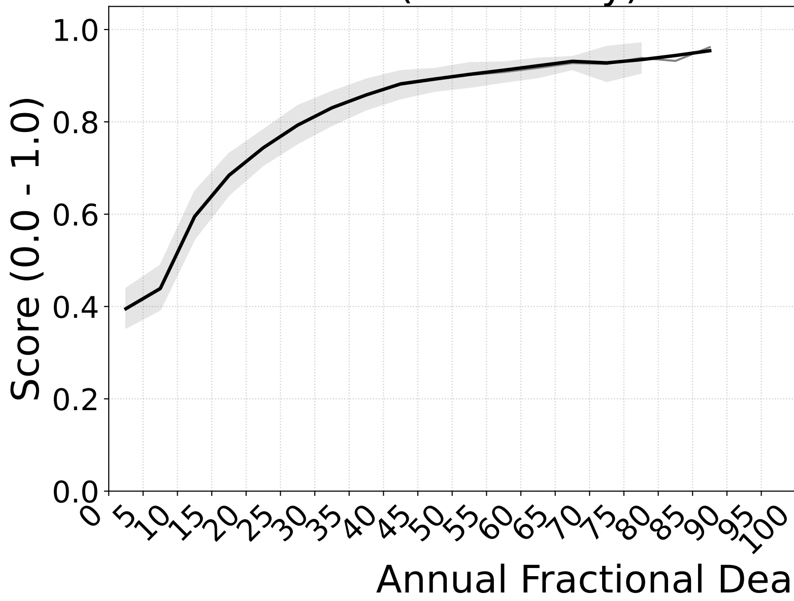
Recall (Sensitivity)
