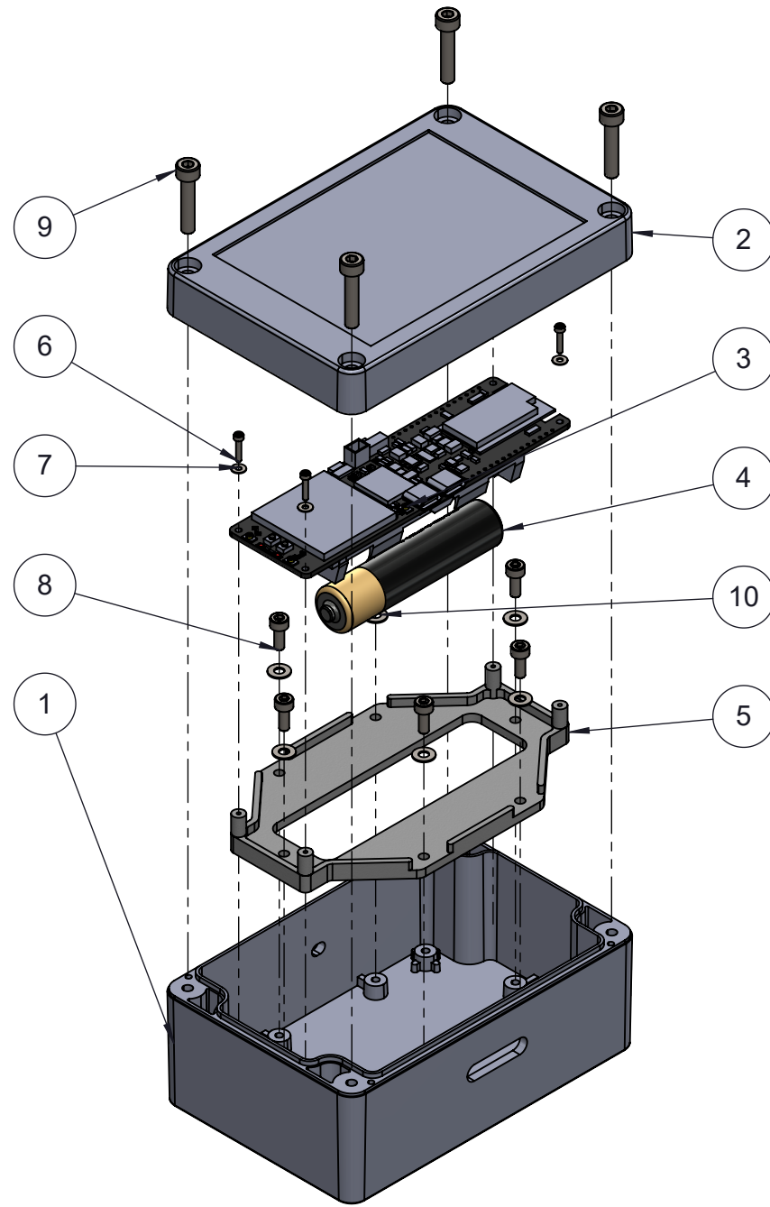
EXPLODED VIEW
