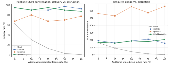
Figure 1: Realistic SGP4 constellation. Left: delivery rate vs. disruption severity. Right: transmission volume (resource usage). CGR-lite and Hybrid-Adaptive (ours) dominate both Naive and Epidemic in delivery rate while using far fewer transmissions, across the full disruption range.
