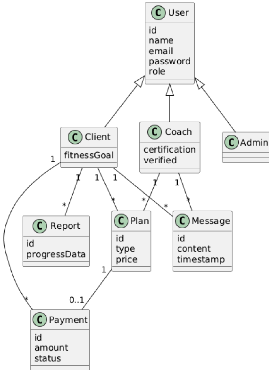
Figure 2: Class Diagram showing system classes and their relationships.
