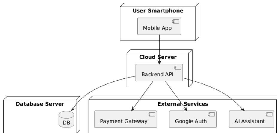
Figure 4: Deployment Diagram showing the hardware and software deployment architecture.
