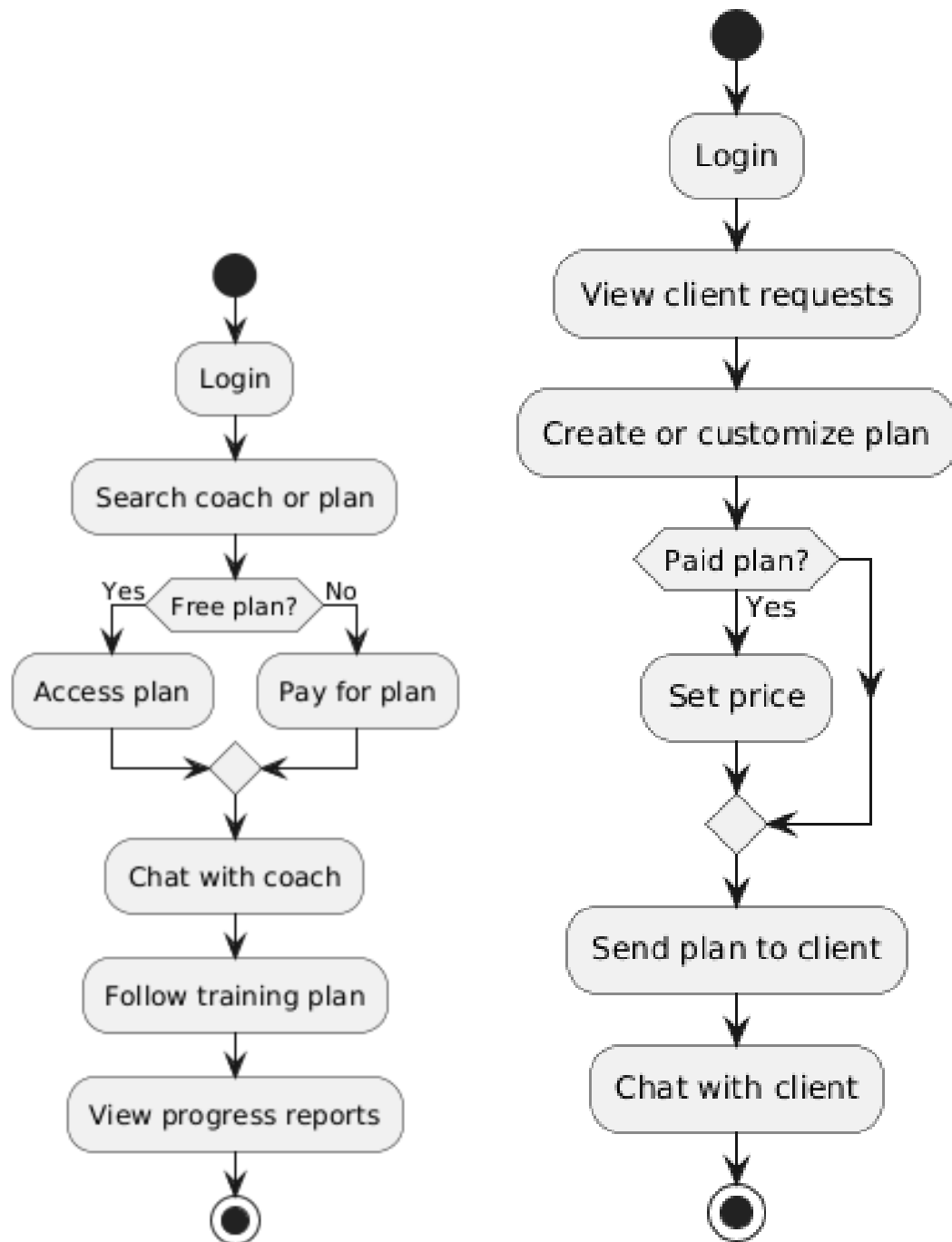
Figure 5: Left: Client Activity Workflow. Right: Coach Activity Workflow.
