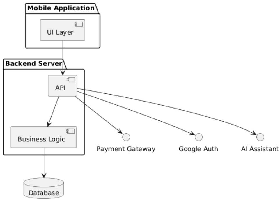
Figure 3: Component Diagram illustrating system modules and dependencies.
