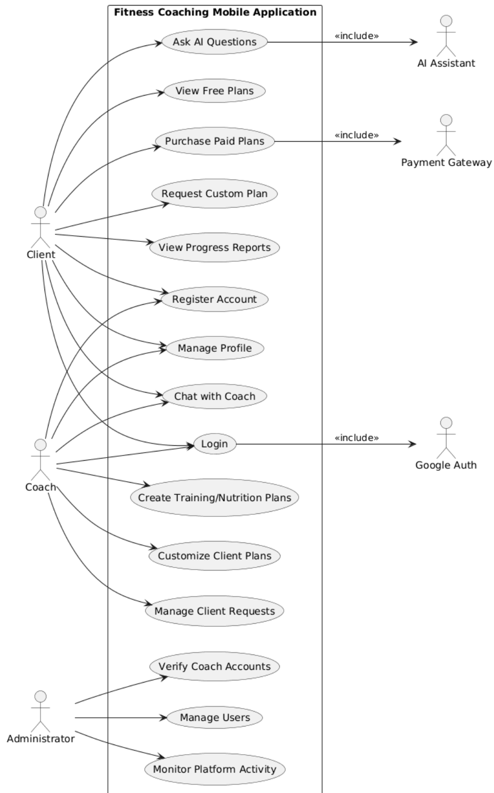
Figure 1: Use Case Diagram showing system actors and interactions.
