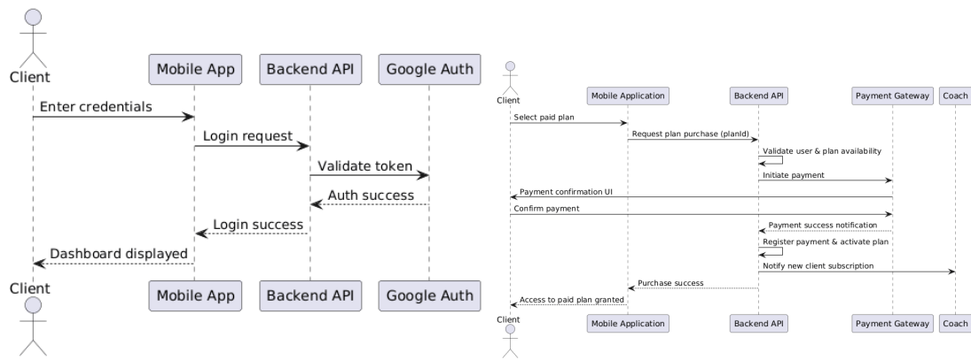
Figure 6: Left: Login Sequence Diagram. Right: Purchase Sequence Diagram.
