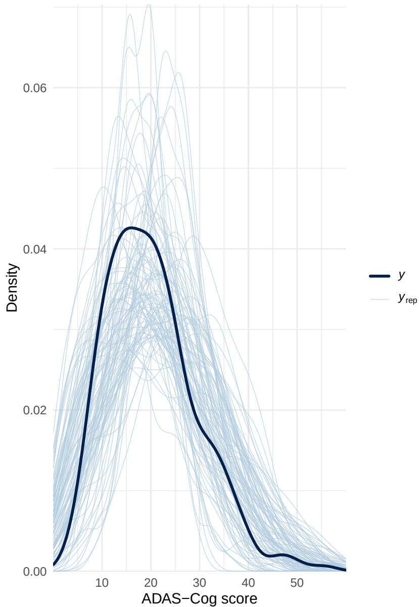
Prior Predictive Check
