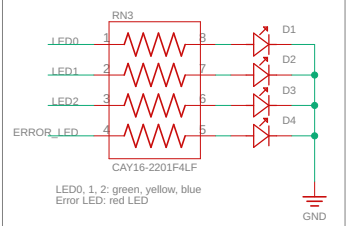
Indicator LEDs
