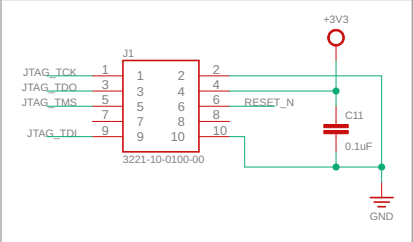
JTAG programming
