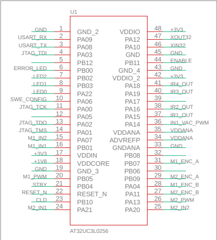
MCU to breakout pins
