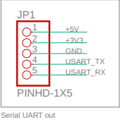
Serial UART out
