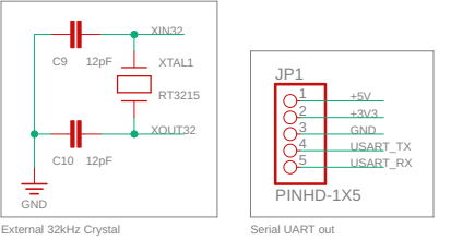
External 32kHz Crystal
