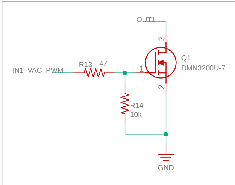
Vacuum Motor Driver
