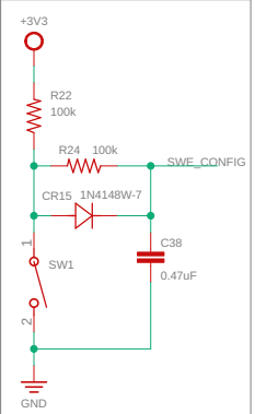
Software Configuration pushbutton
