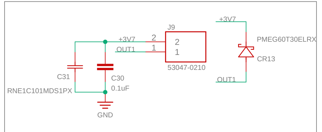
Brushed Motor Picoblade Connector & Flyback Diode
