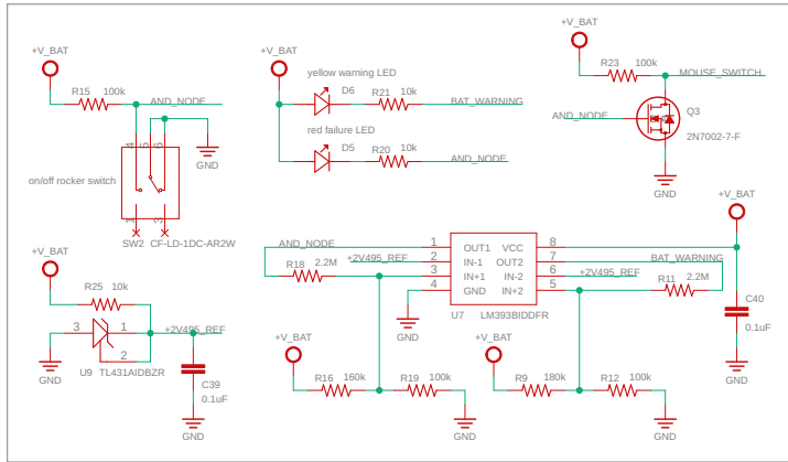
Battery Comparator and Mouse On/Off Switch
