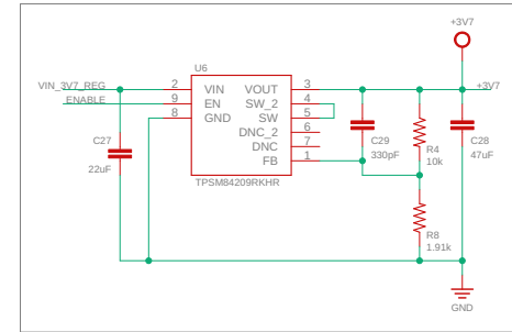
3.7V regulator
