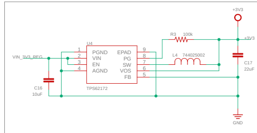
3.3V regulator
