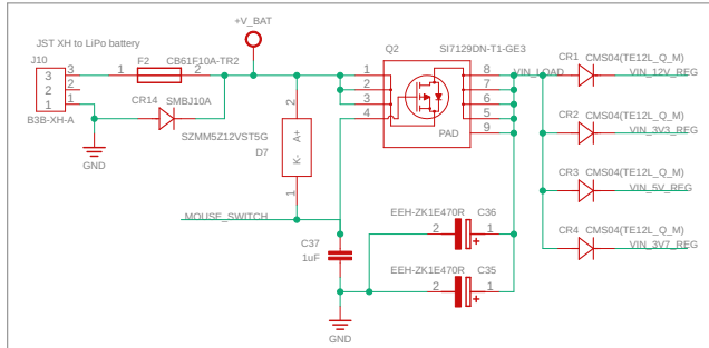
Mouse On/Off Protection
