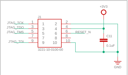
JTAG programming
