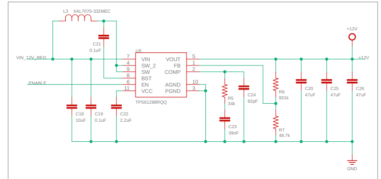
12V regulator
