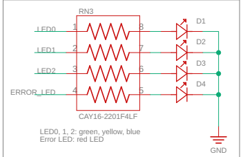
Indicator LEDs
