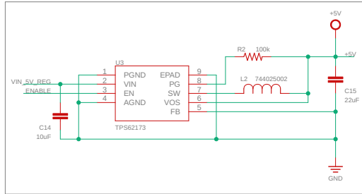
5V regulator
