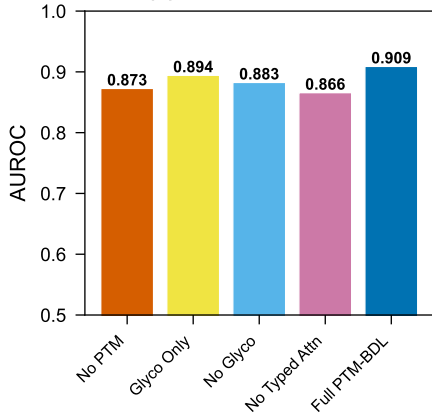
(a) Feature Ablation
