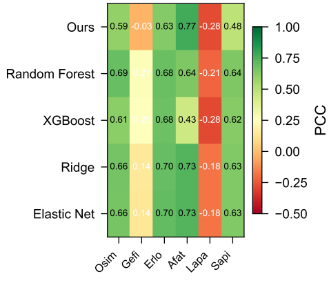
(c) Per-Drug PCC
