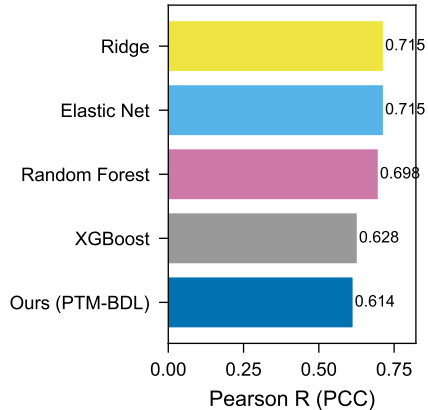
(a) Regression Performance
