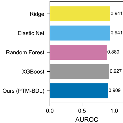
(b) Classification Performance
