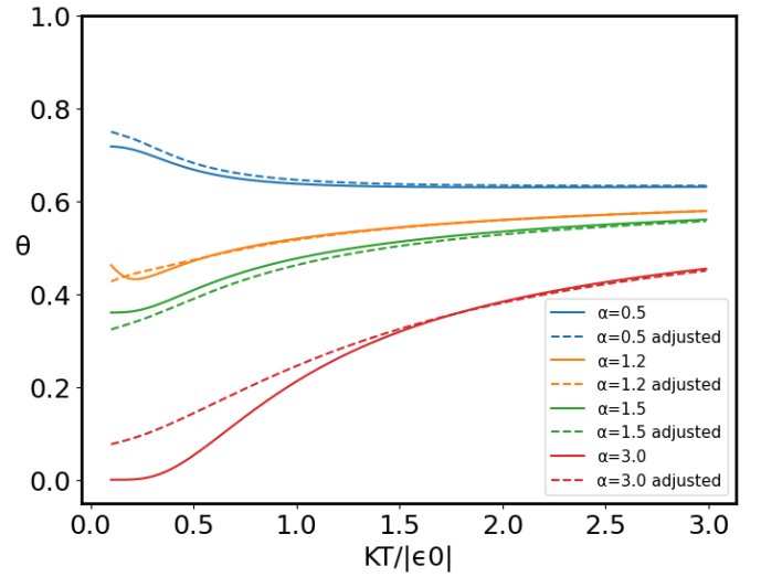
Fig. 4. Helicity \theta(T) for several values of the field-coupling parameter \alpha . Solid lines correspond to the bare prior model, and dashed lines to the geometrically corrected model. The two pipelines agree at high temperature and diverge in the cold regime, with the gap growing with \alpha .
