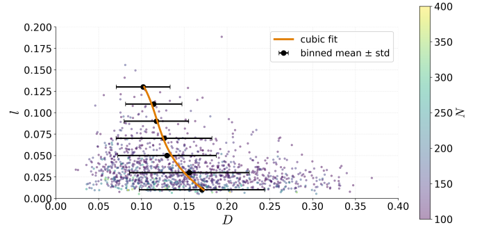
Fig. 2. Scatter plot of average chain height D versus ladder distance l across the SAW sample. Each point corresponds to one self-avoiding walk of length N \geq 100 anchored to the surface. The orange curve is a cubic fit to the binned means; black markers show binned means with standard-deviation error bars.
