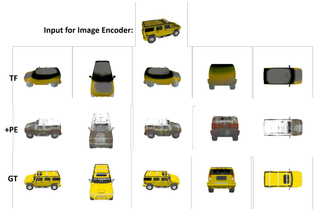
Figure 20. Comparison of novel textures generated after training for 29.5k epochs on five car models. The models are given as input the shape- and image-encodings from a previously unseen car, and then predict a corresponding texture. The image-encoding is calculated from a single view of the car, which is displayed at the top of the figure. As expected, neither model did particularly well at this task due to limited training; however, ORIG better approximated the color of the target texture, seeming to appropriately lift the coloring-scheme of the yellow-car from the training set. On extremely close inspection, it's apparent both models made slight attempts at the lettering on the windshield of the truck, with the PE model's version slightly more pronounced.
