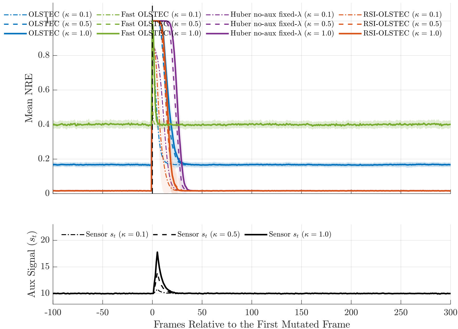
(a) Tracking Response to Controlled Subspace Changes
