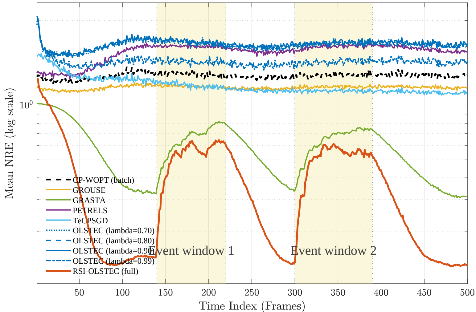
S3 LNE Gaussian-Spatter Benchmark with Smooth Dynamics and Event Changes (n=50)
