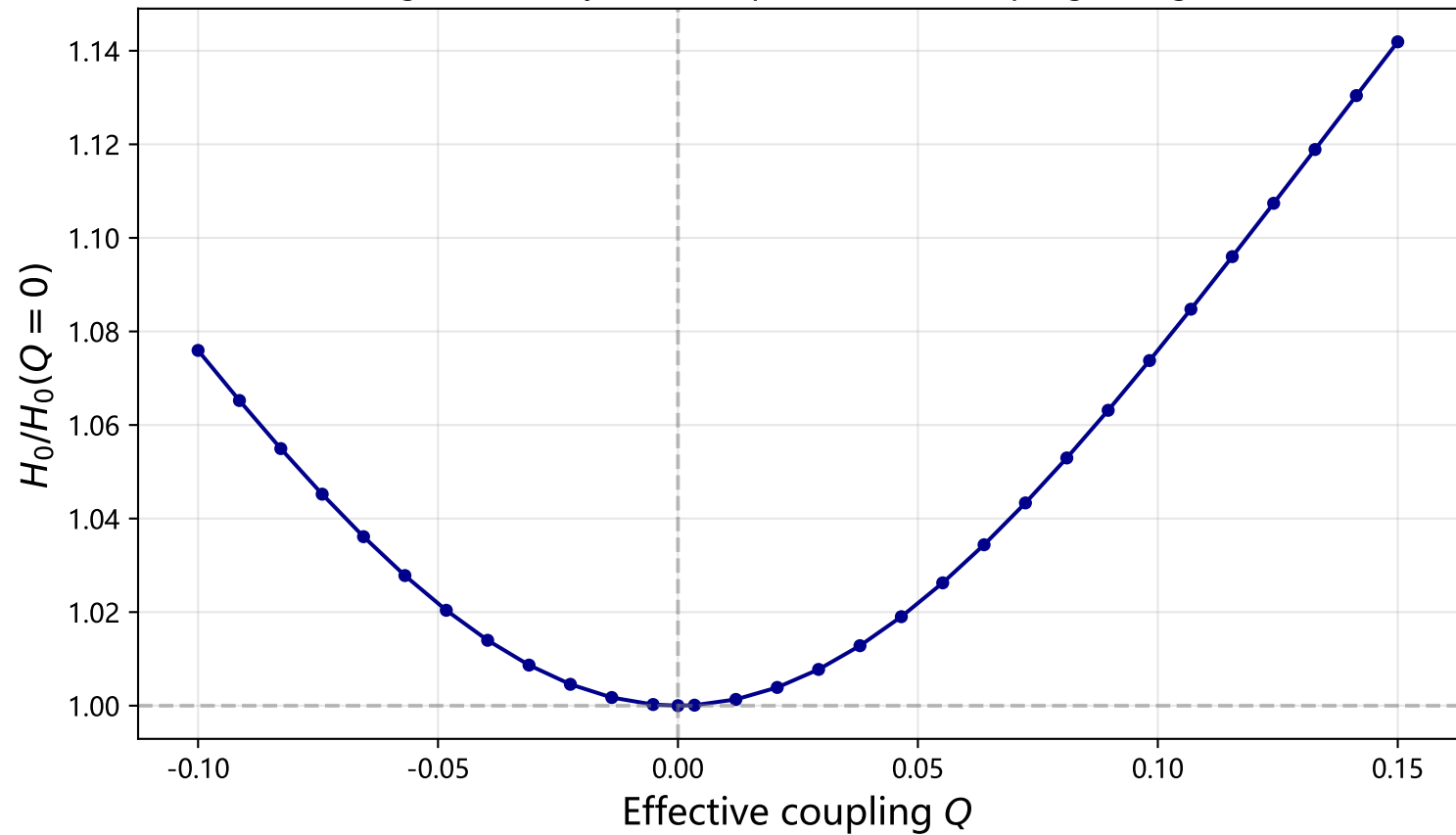
Figure 3: Today's Hubble parameter vs coupling strength
