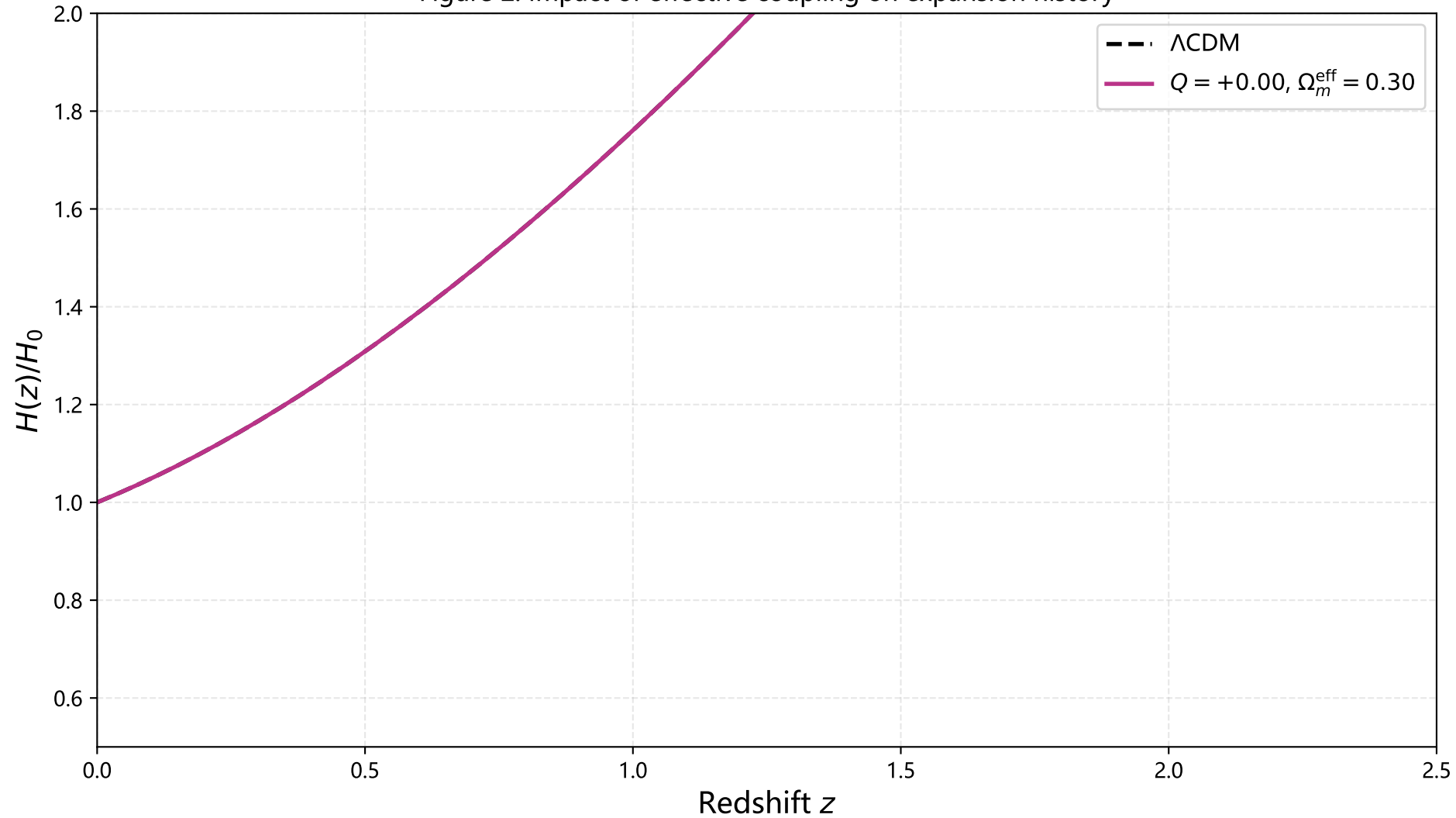
Figure 2: Impact of effective coupling on expansion history
