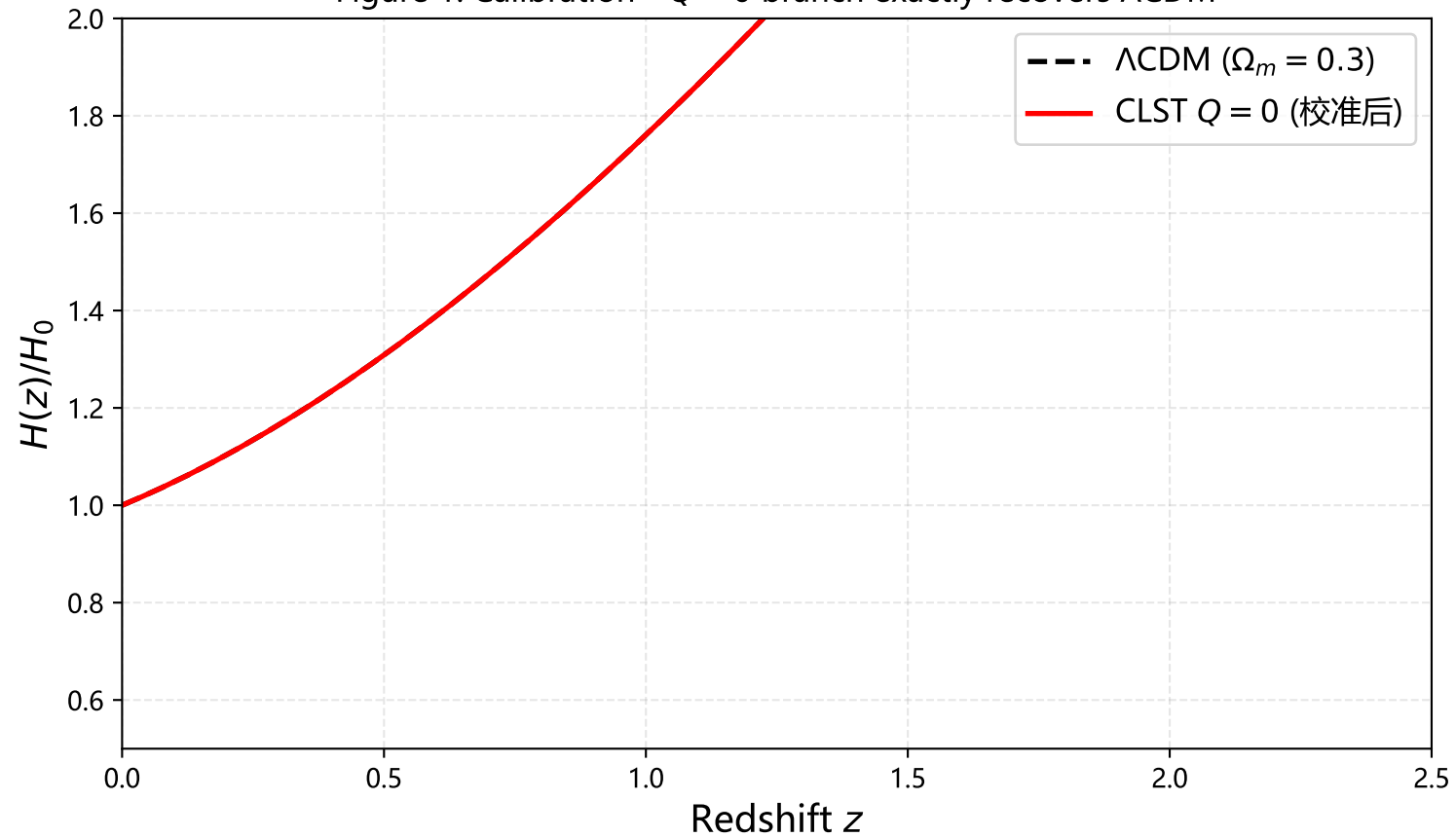
Figure 1: Calibration - Q = 0 branch exactly recovers \Lambda CDM
