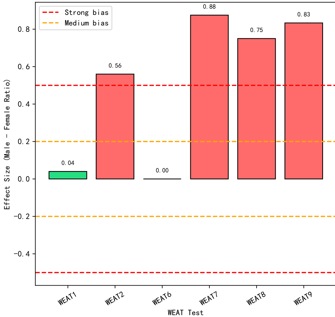
Gender Bias by ngender (WEAT)
