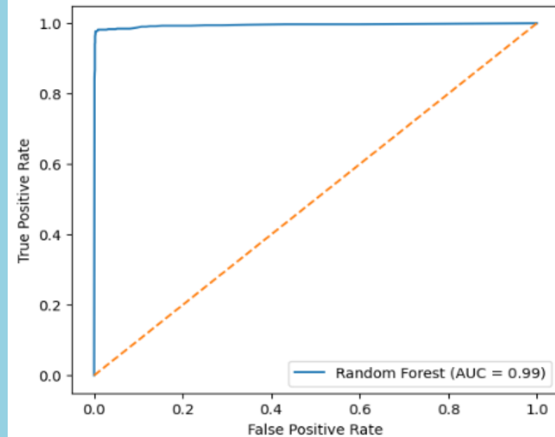
ROC Curve - Random Forest
