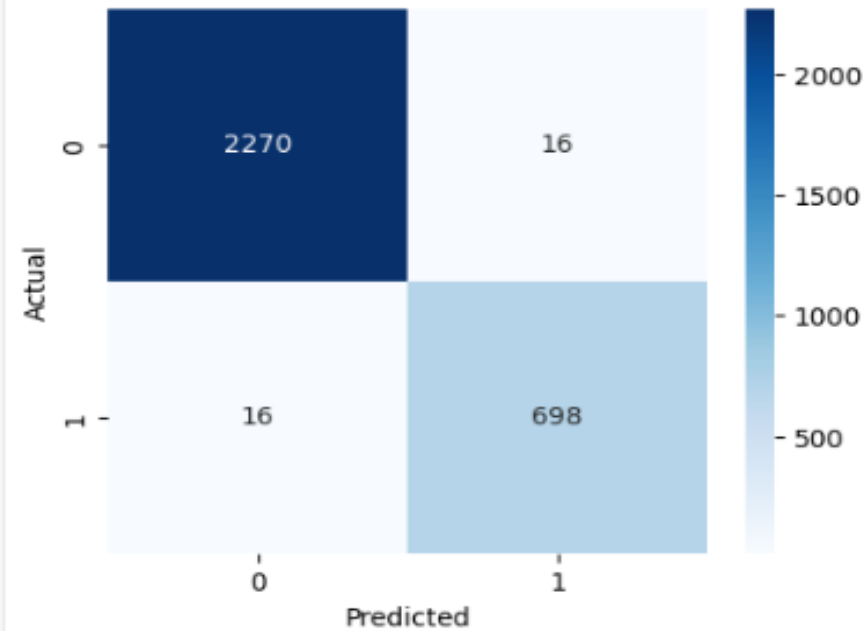
Confusion Matrix - Random Forest
