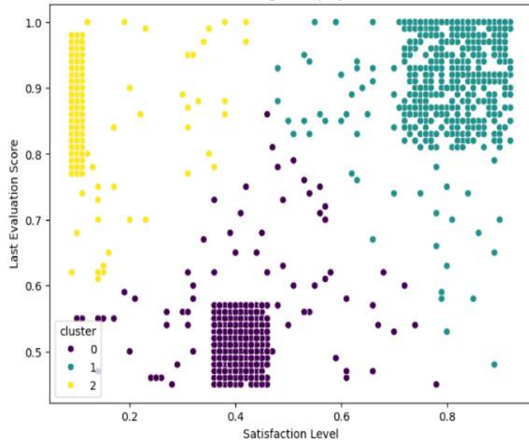
K-Means Clustering of Employees Who Left
