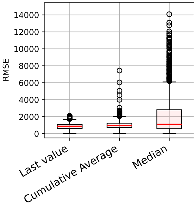
RMSE for Infected, group 1
