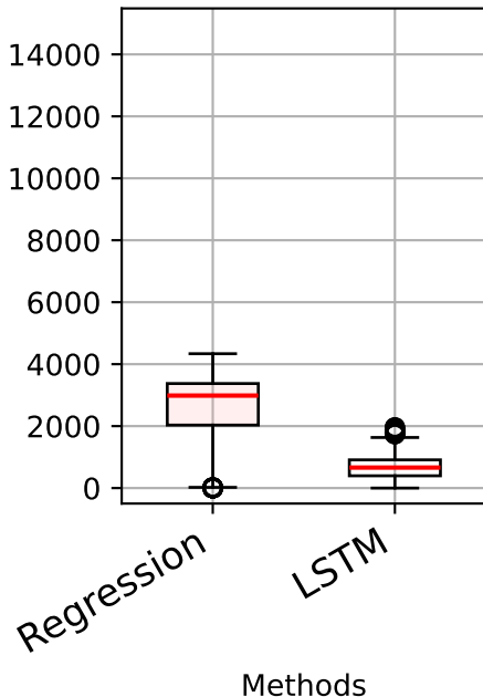
RMSE for Infected, group 2
