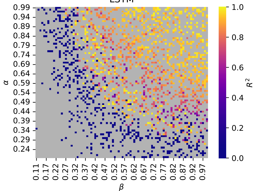
LSTM
