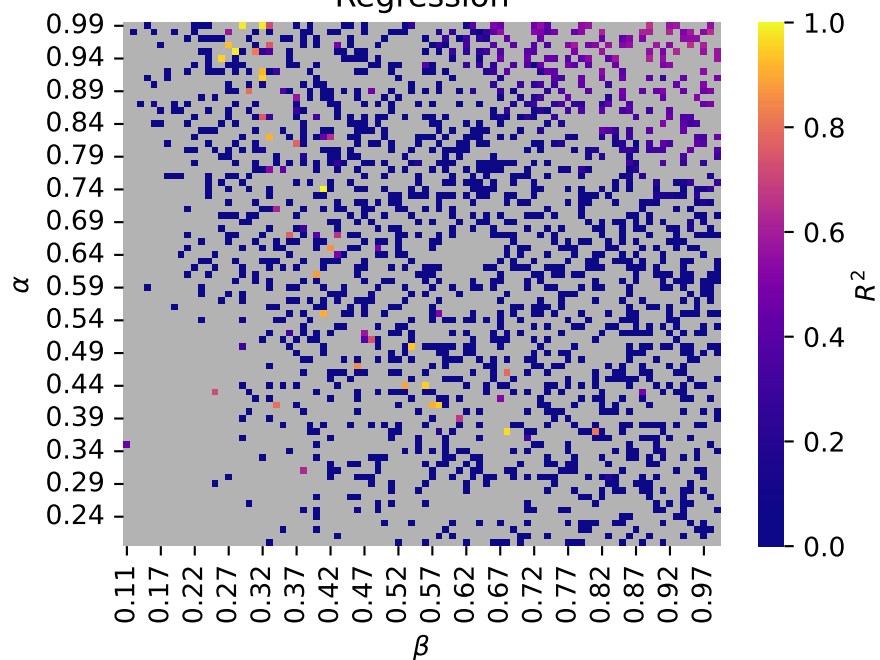
Regression
