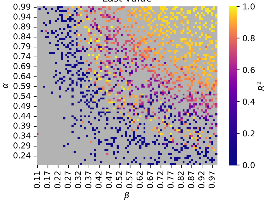
Last value
