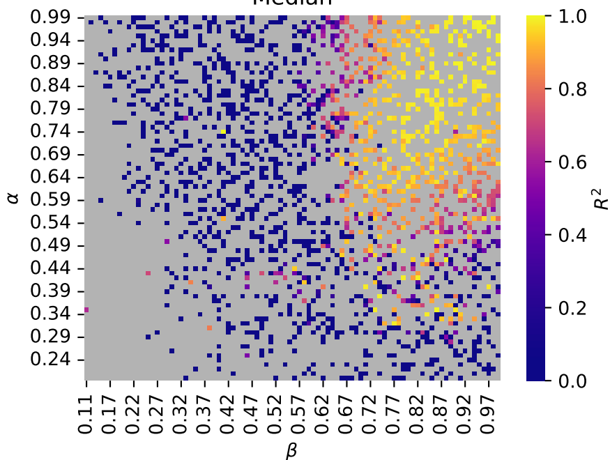
Median
