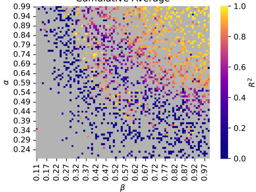
Cumulative Average
