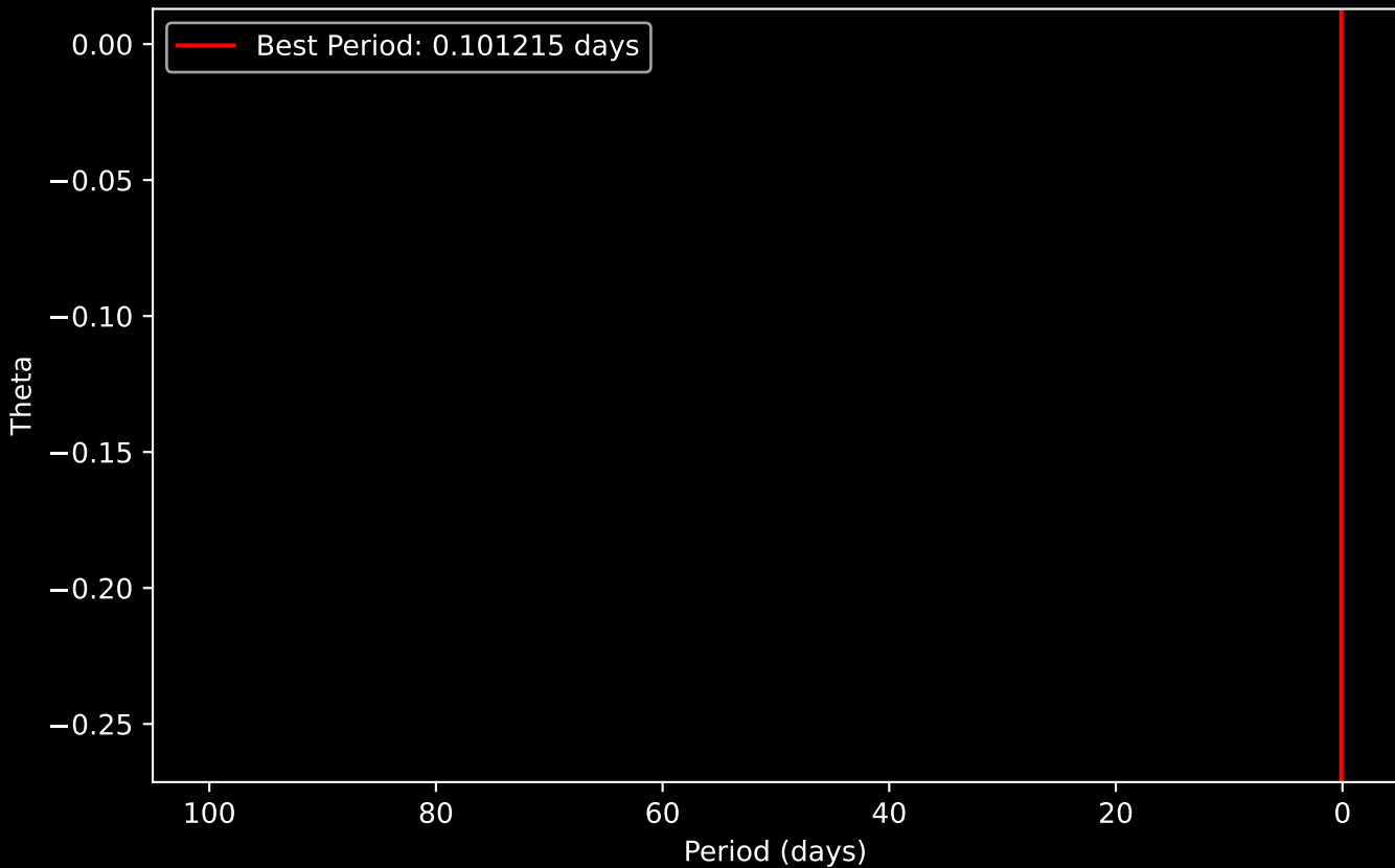
PDM Plot of the Star with ID 6730764715540788352
