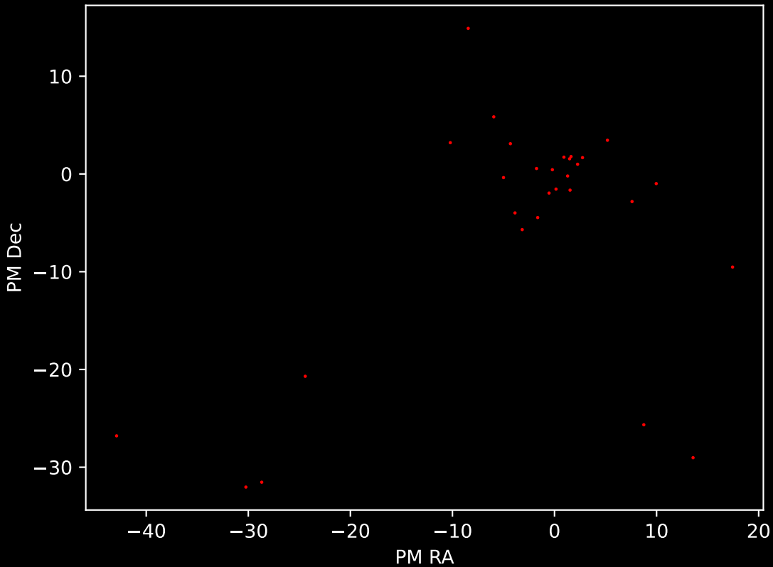
PMRA vs PMDEC MiMes Survey Data
