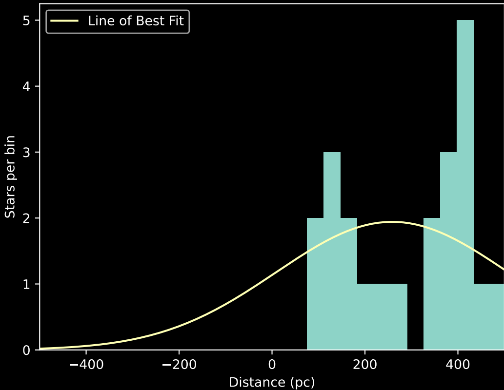
Fitted Histogram MiMes Survey Data
