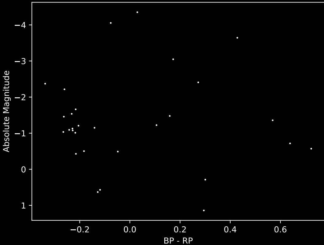
HR Diagram MiMes Survey Data
