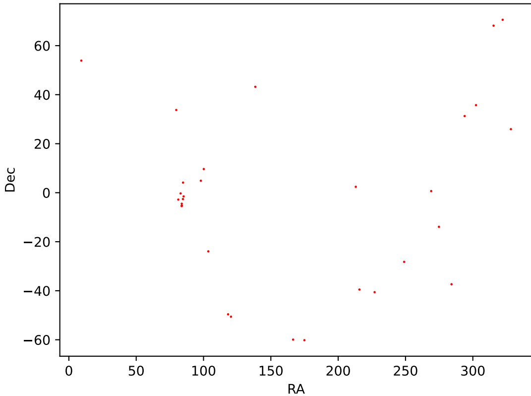
RA vs Dec MiMes Survey Data
