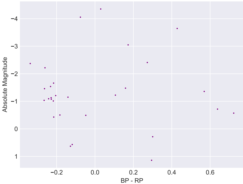
Hertzsprung-Russell Diagram
