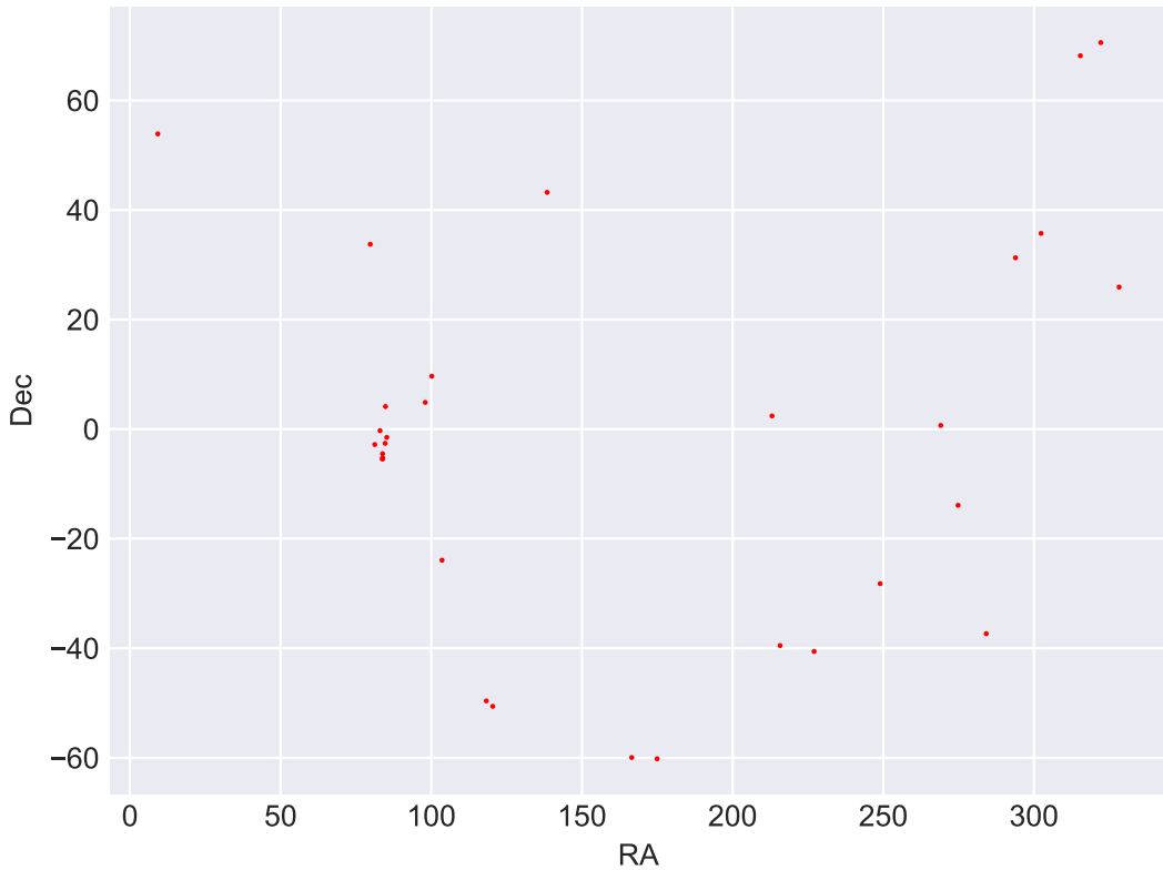
Right Ascension Vs. Declination
