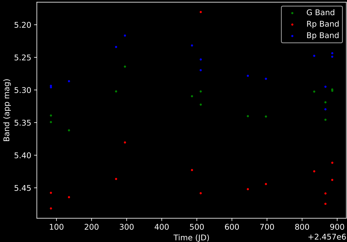
Flux vs Time of the Star with ID 6730764715540788352
