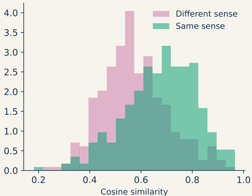
BERT mean last 4
