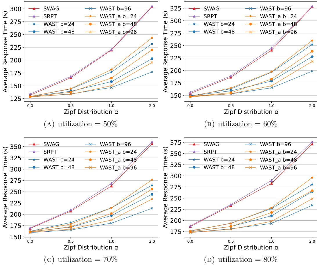
FIGURE 4.7: Average Job Response Time, Alibaba 2018
