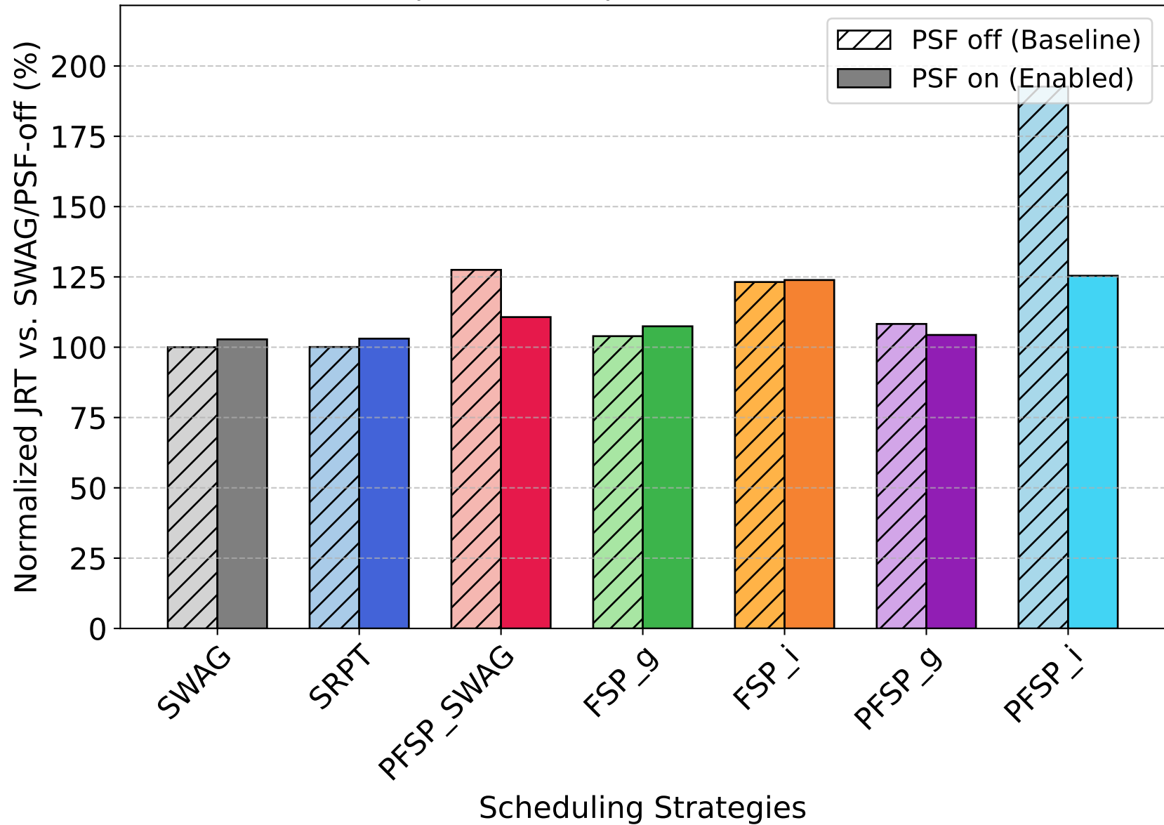
Comparison at Zipf Distribution \alpha = 0.0
