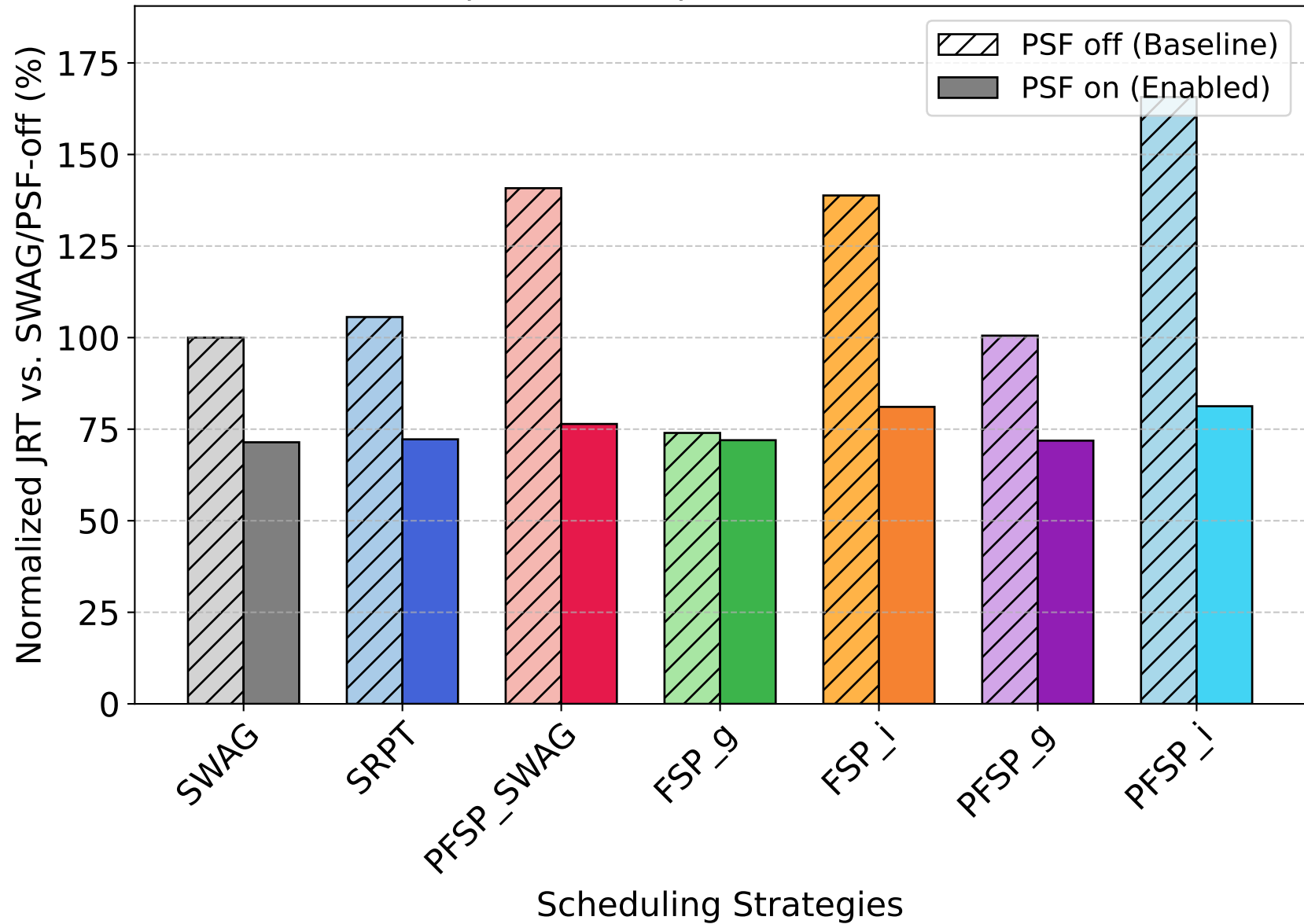
Comparison at Zipf Distribution \alpha = 0.5
