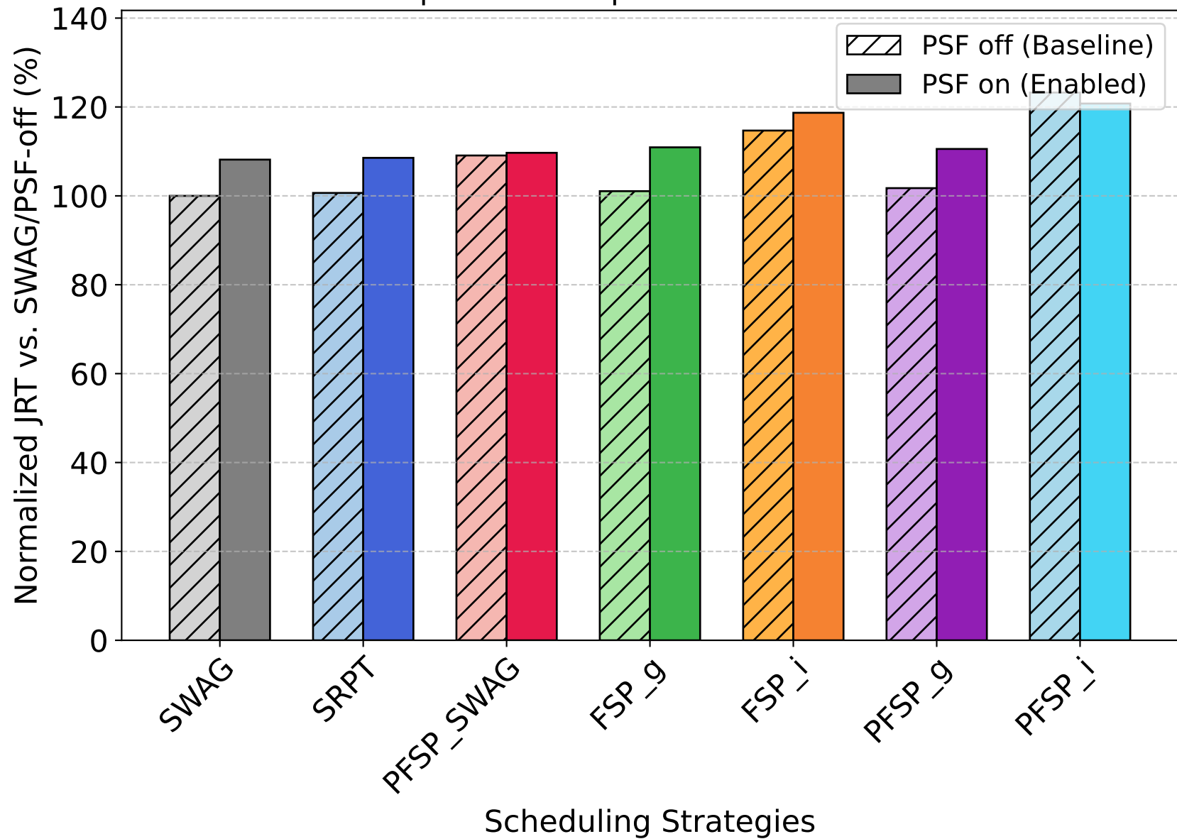
Comparison at Zipf Distribution \alpha = 0.0
