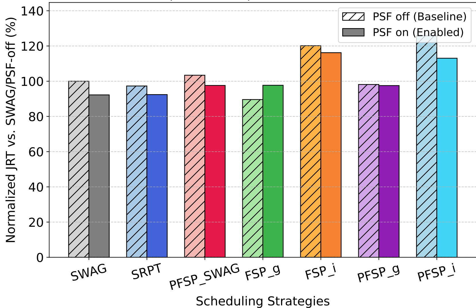
Comparison at Zipf Distribution \alpha = 1.0
