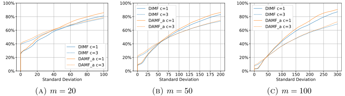
FIGURE 3.11: Cumulative distribution of standard deviation, Alibaba, workload = 40%, Zipf parameter \alpha = 1
