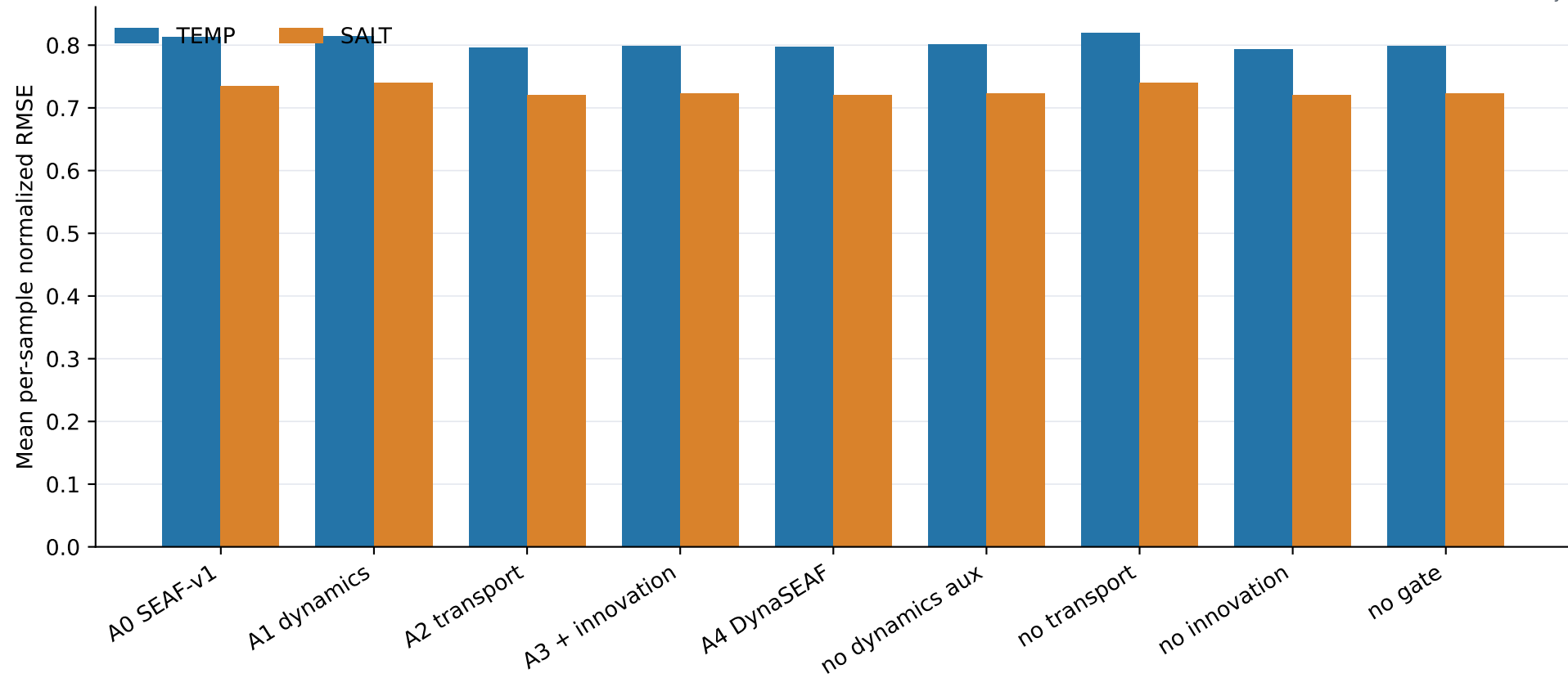
DynaSEAF validation ablation screen (seed 42)
