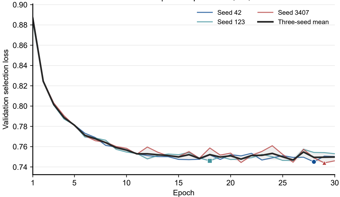
FourCastNet | best epochs: 28, 18, 29
