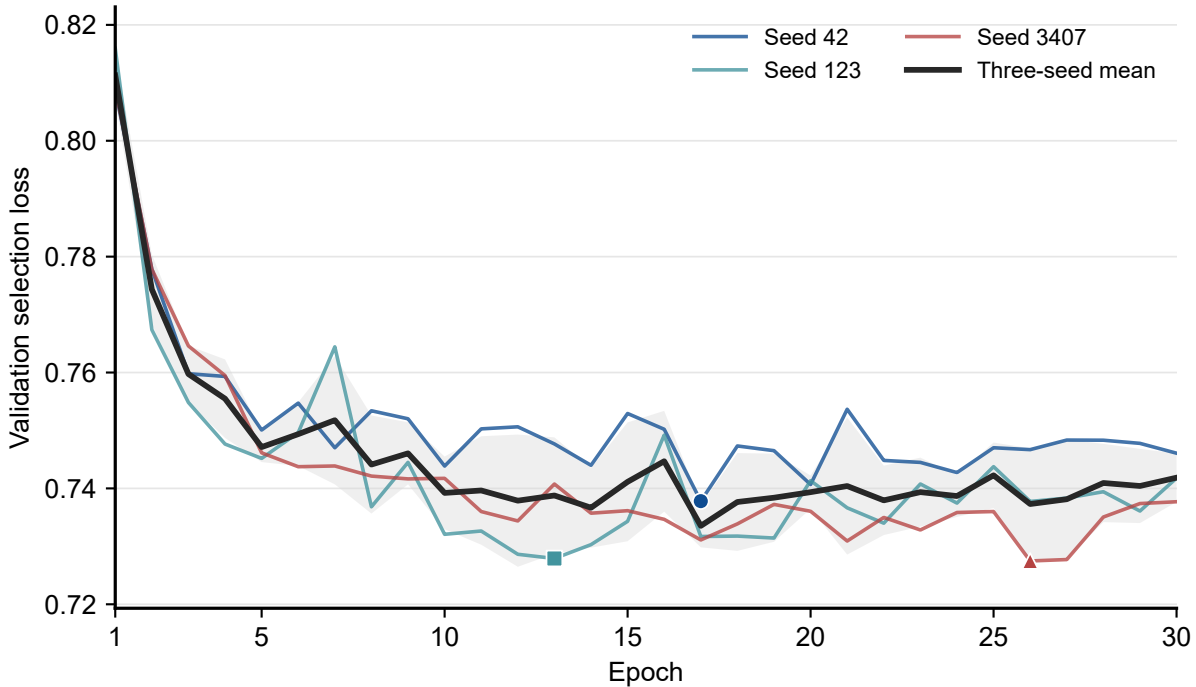
Swin | best epochs: 17, 13, 26
