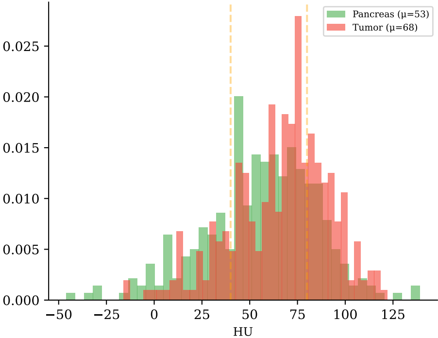
HU Distribution
