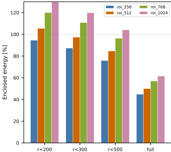
(a) PSF ROI Energy Decomposition | noise-floor vs diffraction wing separation
