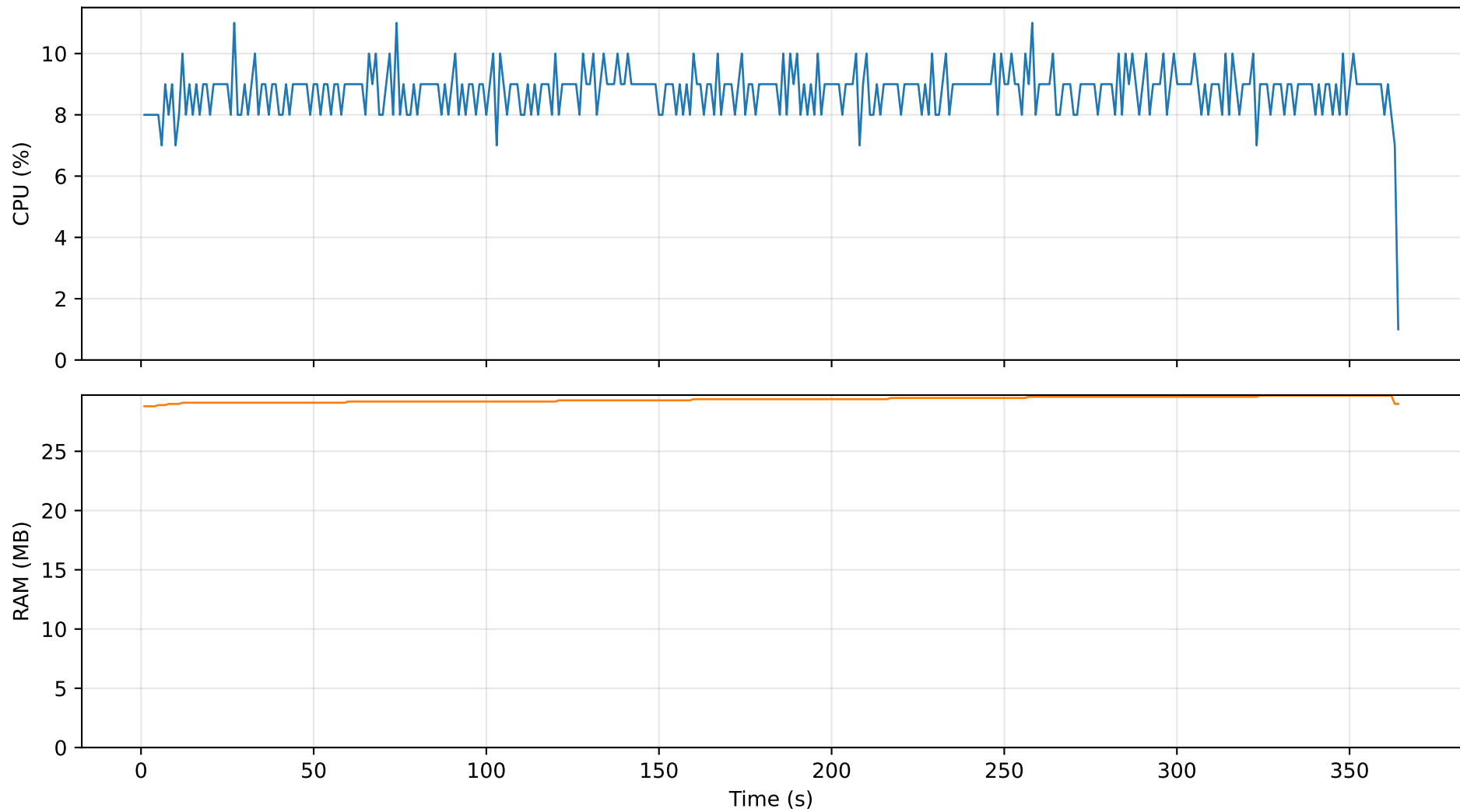
Resource Usage — 10pct_007
