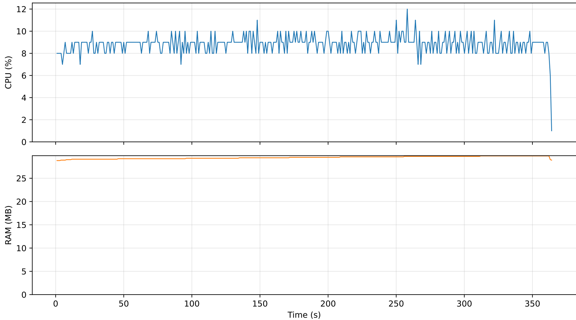
Resource Usage — 20pct_002
